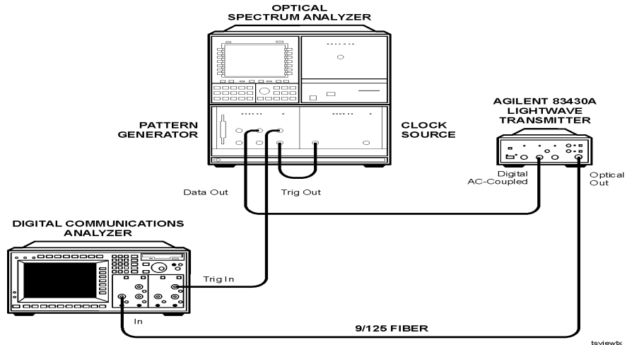
Figure 5-8. Equipment setup for eye quality
