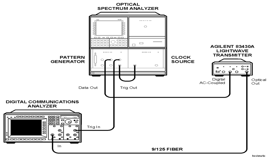
Figure 5-13. Equipment setup for laser bias
