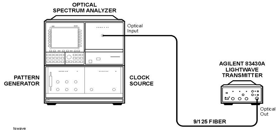
Figure 5-10. Equipment setup for output wavelength
