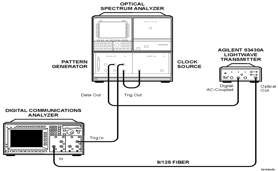
Figure 5-7. Equipment setup for eye quality
