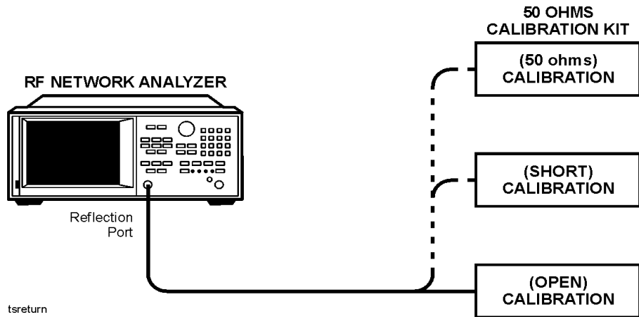
Figure 5-4. Calibration kit connections
